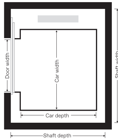
Shaft plan (side opening)
