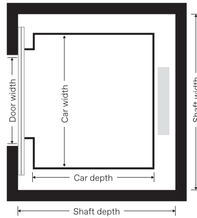
Shaft plan (centre opening)
