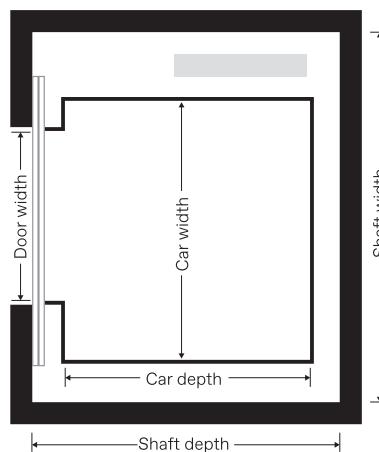
Shaft plan (centre opening)
