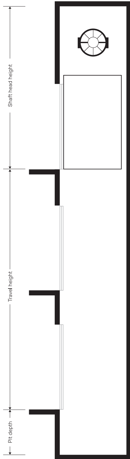
Shaft vertical section
